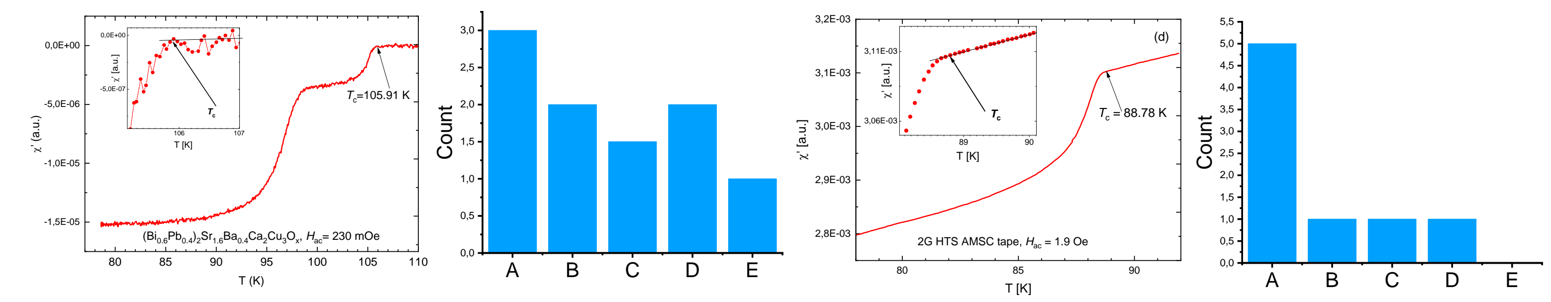
Fig 4. Other examples of \chi' measurements and associated word occurrences histograms. Insets show the critical temperature T_c of a sample.
