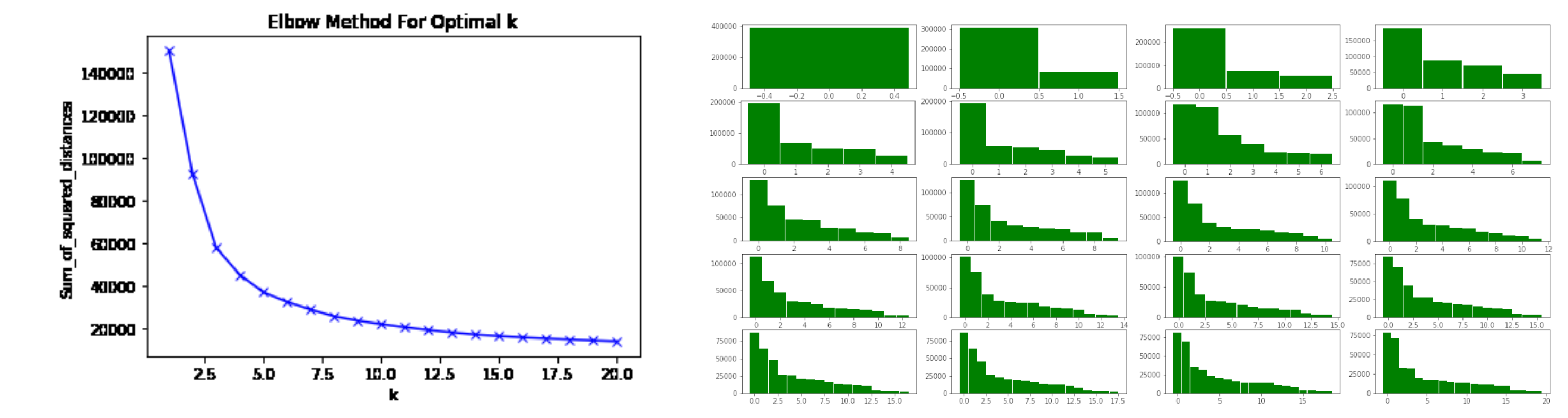
Fig 5. Estimation of the optimal cluster number for k-means algorithm. Left graph - The elbow method for an optimal K estimation, right graph - number of clusters and resulting clusters sizes.
