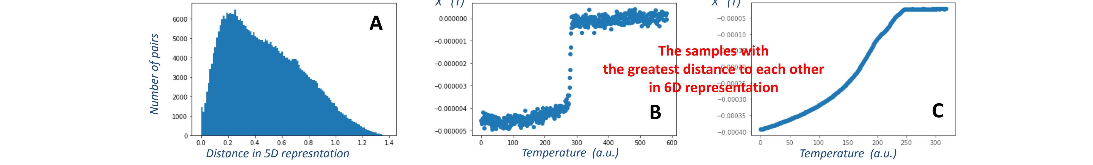
Fig 10. A) Distances between all possible pairs of two \chi'(T) measurements. B) \chi'(T) for a HTS wire (high value of critical current density, sharp SC transition) C) \chi'(T) for grinded and pressed into a pellet polycrystalline REBCO-123 (electric current can not flow, wide SC transition)
